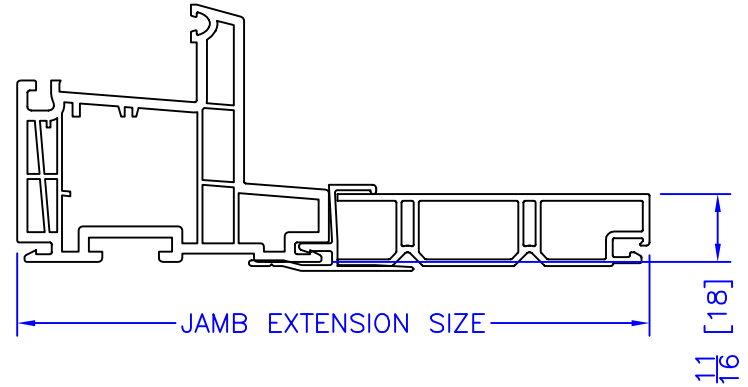
JAMB EXTENSION CLADDED
