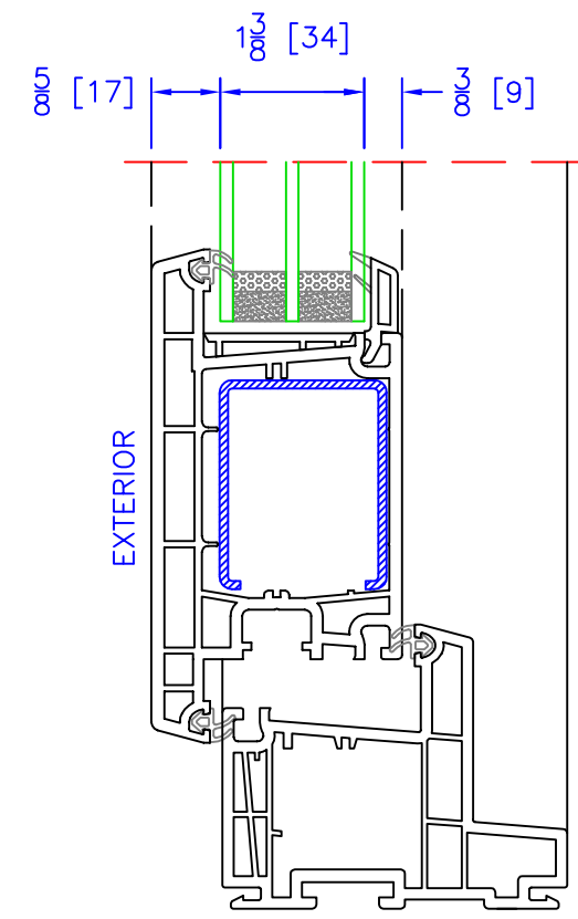
OUTSWING SASH TRIPLE GLAZING OPTION ( 1\frac{3}{8} " OA)
