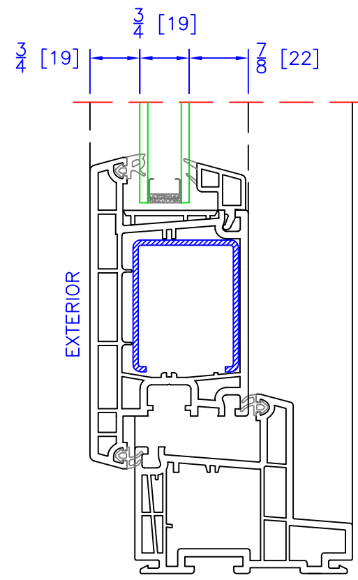
OUTSWING SASH DUAL GLAZING OPTION ( \frac{3}{4} " OA)
