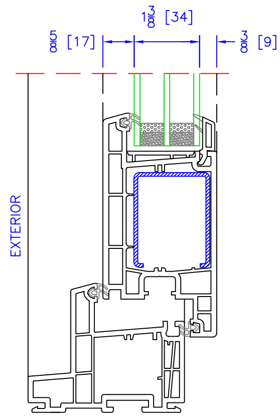
INSWING SASH TRIPLE GLAZING OPTION ( 1\frac{3}{8} " OA)
