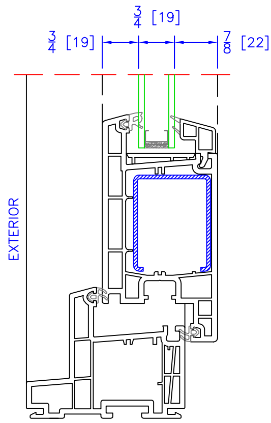
INSWING SASH DUAL GLAZING OPTION ( \frac{3}{4} " OA)
