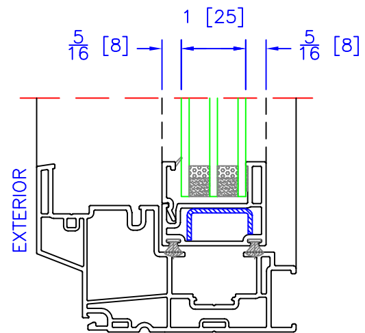
OPERATING SASH TRIPLE GLAZING OPTION (1" OA)
