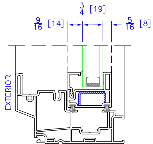
OPERATING SASH DUAL GLAZING OPTION ( \frac{3}{4} " OA)
