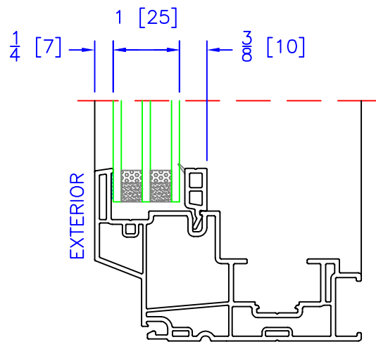
FIXED TRIPLE GLAZING OPTION (1" OA)
