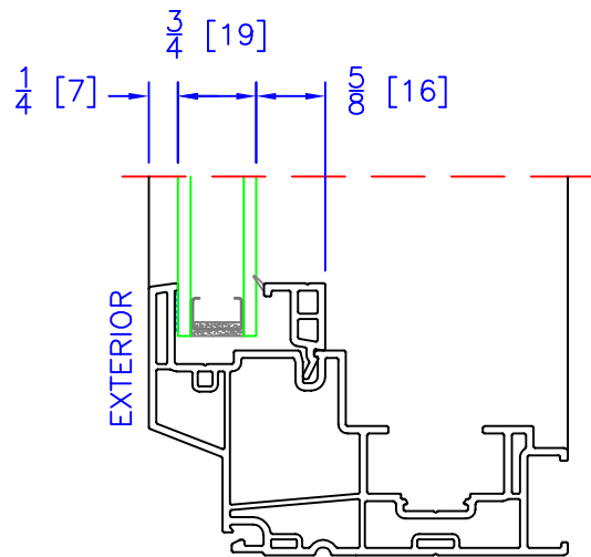
FIXED DUAL GLAZING OPTION ( \frac{3}{4} " OA)
