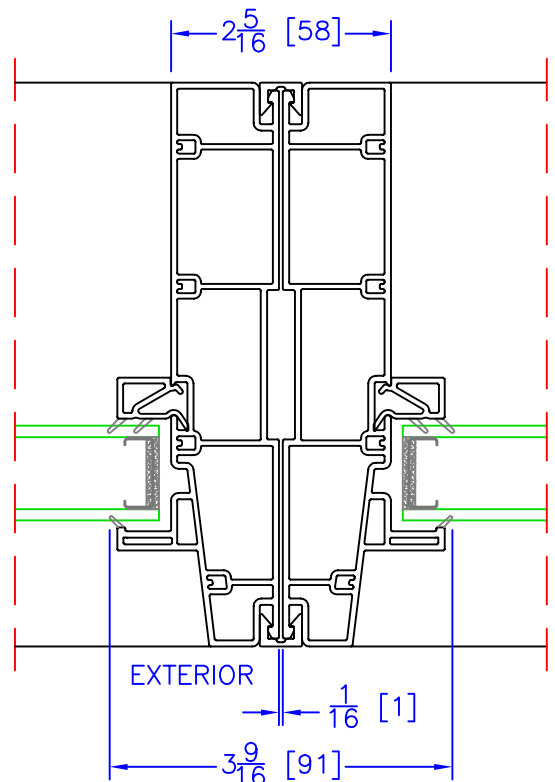
TRANSOM/TRANSOM VERTICAL MULLION
