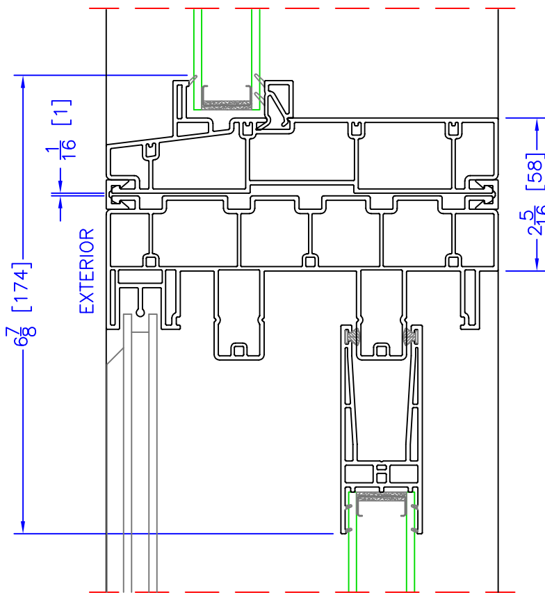
TRANSOM/OPERATOR HORIZONTAL MULLION
