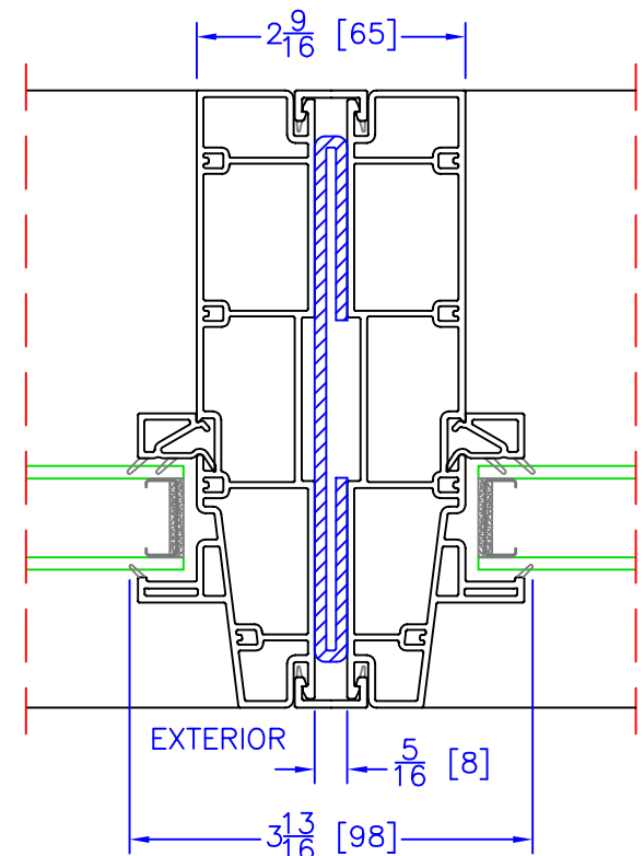
TRANSOM/TRANSOM VERTICAL REINFORCEMENT MULLION
