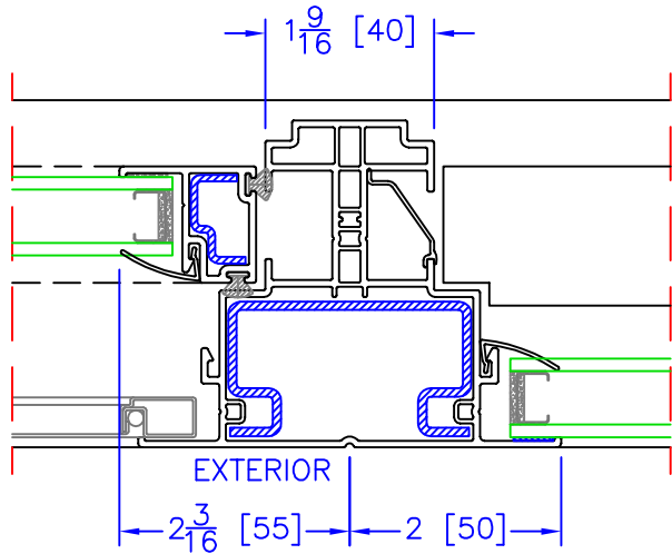
OPERATOR (BOTTOM SASH)/FIXED VERTICAL T-MULLION
