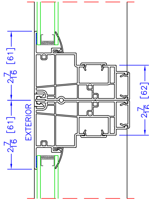
FIXED/OPERATOR OR FIXED HORIZONTAL MULLION
