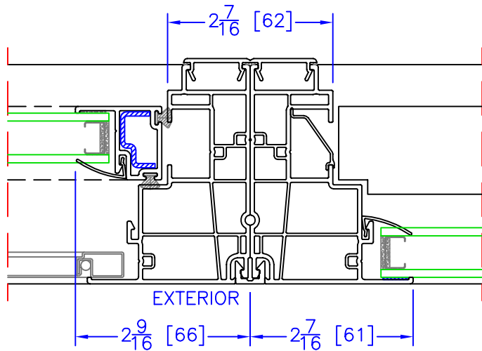
OPERATOR (BOTTOM SASH)/FIXED VERTICAL MULLION
