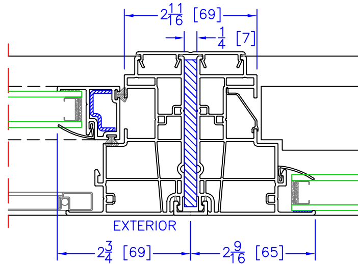
OPERATOR (BOTTOM SASH)/FIXED VERTICAL REINFORCEMENT MULLION
