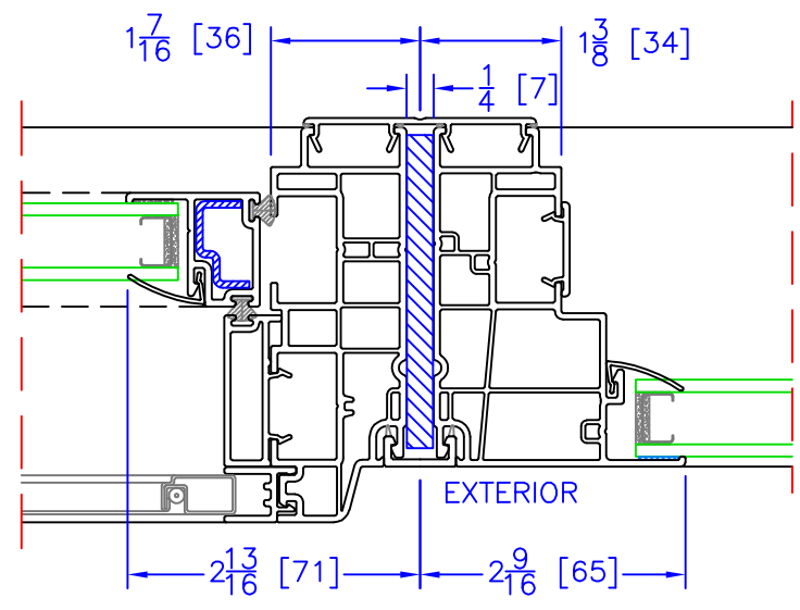
OPERATOR (BOTTOM SASH)/FIXED VERTICAL REINFORCEMENT MULLION
