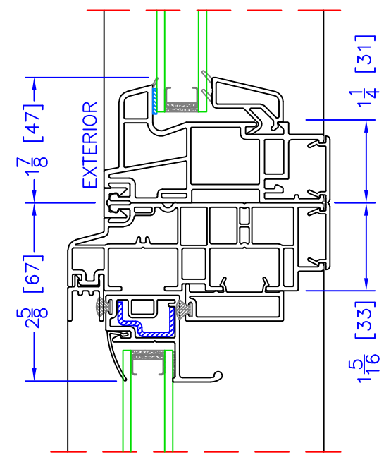
SHAPE/OPERATOR HORIZONTAL MULLION
