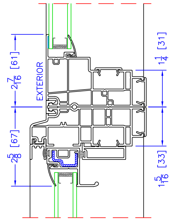
FIXED/OPERATOR HORIZONTAL MULLION
