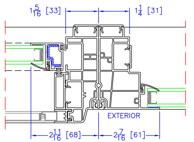
OPERATOR (BOTTOM SASH)/FIXED VERTICAL MULLION
