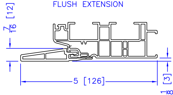
FLUSH EXTENSION
