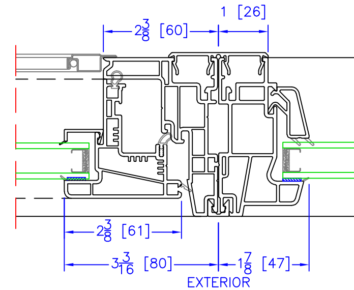
OPERATOR/NARROW PICTURE (PN) VERTICAL/HORIZONTAL MULLION
