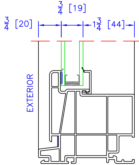
WIDE PICTURE (PW) DUAL GLAZING OPTION ( \frac{3}{4} " OA)
