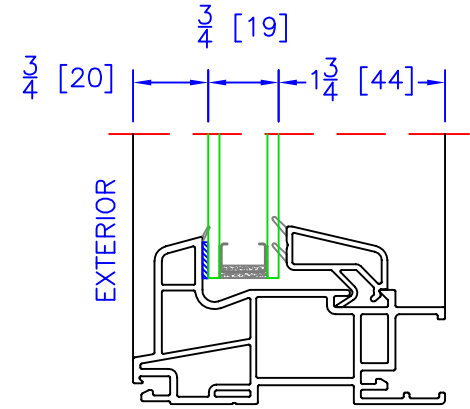
NARROW PICTURE (PN) DUAL GLAZING OPTION ( \frac{3}{4} " OA)
