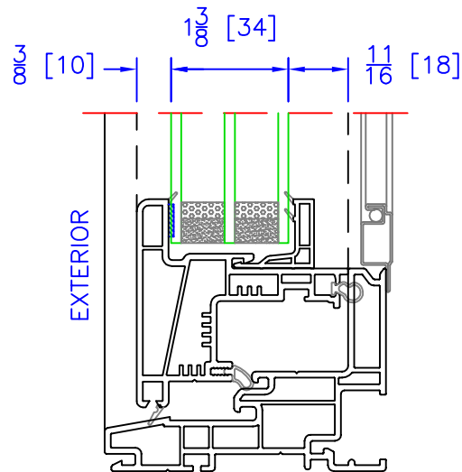
OPERATOR/FIXED TRIPLE GLAZING OPTION ( 1\frac{3}{8} " OA)
