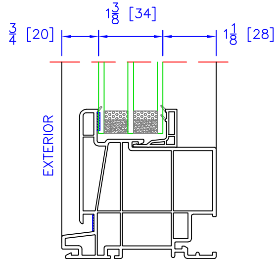
WIDE PICTURE (PW) TRIPLE GLAZING OPTION ( 1\frac{3}{8} " OA)
