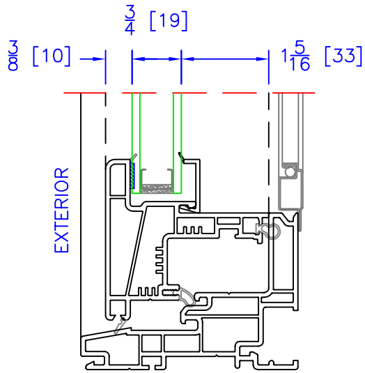
OPERATOR/FIXED DUAL GLAZING OPTION ( \frac{3}{4} " OA)
