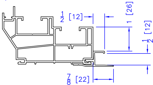
1/2" ADD ON DRYWALL RETURN
