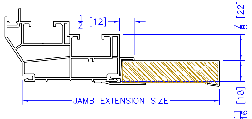
JAMB EXTENSION PRIMED
