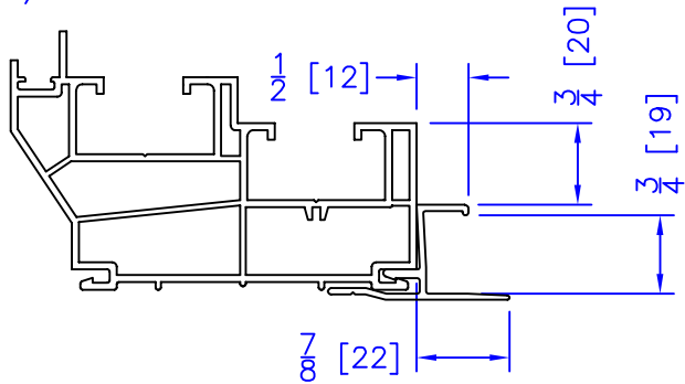
3/4" ADD ON DRYWALL RETURN
