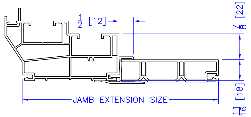
JAMB EXTENSION CLADDED
