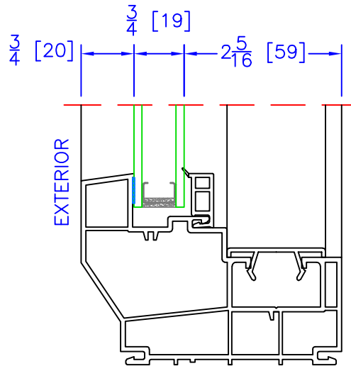
FIXED DUAL GLAZING OPTION ( \frac{3}{4} " OA)
