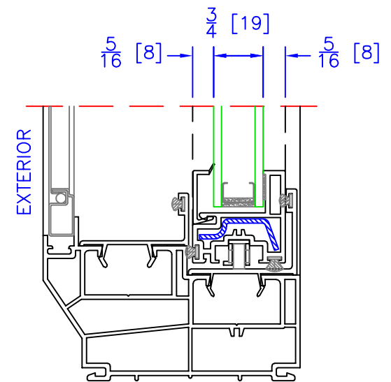
DOUBLE GLIDER INSIDE SASH DUAL GLAZING OPTION ( \frac{3}{4} " OA)
