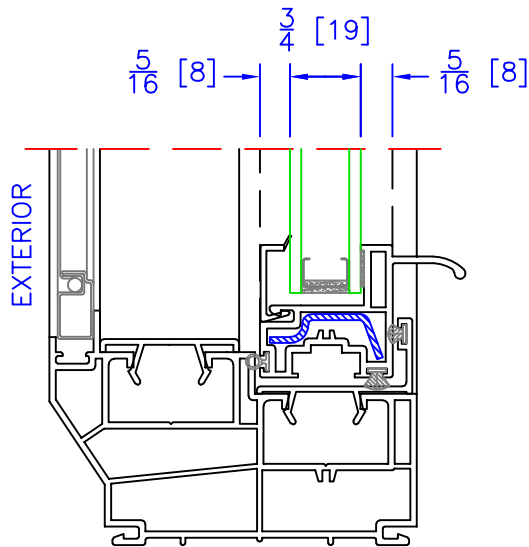
DOUBLE HUNG BOTTOM SASH DUAL GLAZING OPTION ( \frac{3}{4} " OA)
