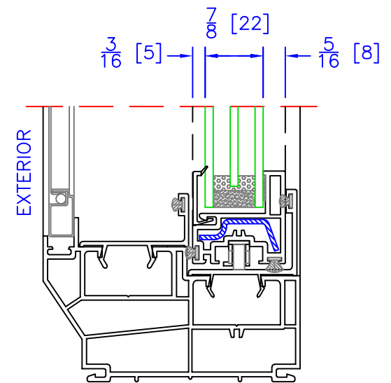
DOUBLE GLIDER INSIDE SASH TRIPLE GLAZING OPTION ( \frac{7}{8} " OA)
