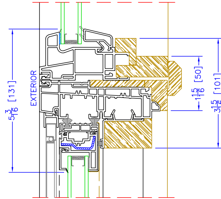
TRANSOM/OPERATOR HORIZONTAL MULLION
