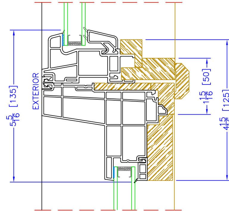
TRANSOM/FIXED HORIZONTAL MULLION
