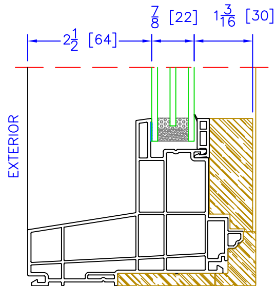
FIXED TRIPLE GLAZING OPTION ( \frac{7}{8} " OA)
