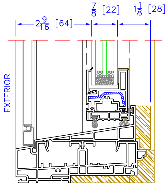
OPERATOR TRIPLE GLAZING OPTION ( \frac{7}{8} " OA)
