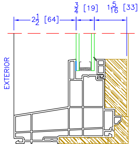
FIXED DUAL GLAZING OPTION ( \frac{3}{4} " OA)
