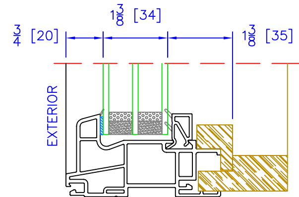
TRANSOM TRIPLE GLAZING OPTION ( 1\frac{3}{8} " OA)
