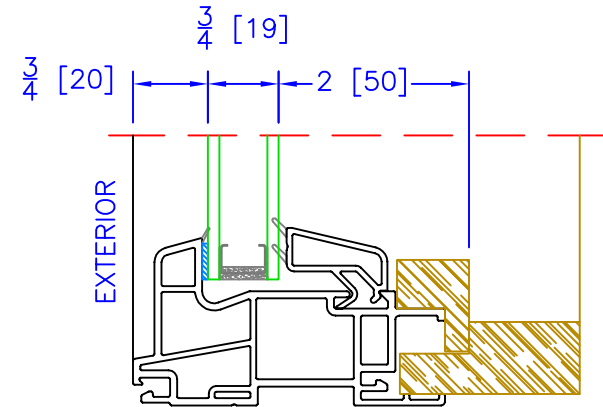
TRANSOM DUAL GLAZING OPTION ( \frac{3}{4} " OA)
