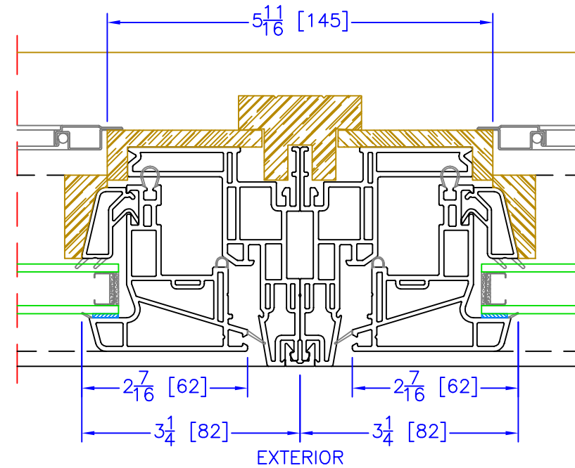
OPERATOR/OPERATOR VERTICAL/HORIZONTAL MULLION
