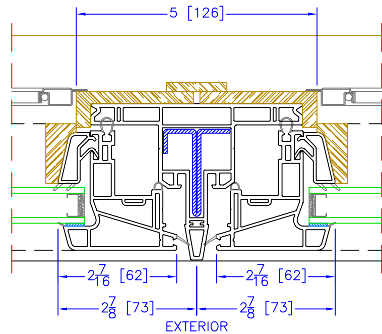
OPERATOR/OPERATOR VERTICAL/HORIZONTAL T-MULLION
