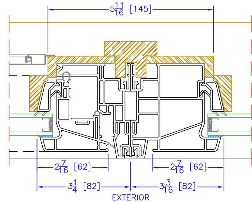
OPERATOR/WIDE PICTURE (PW) VERTICAL/HORIZONTAL MULLION
