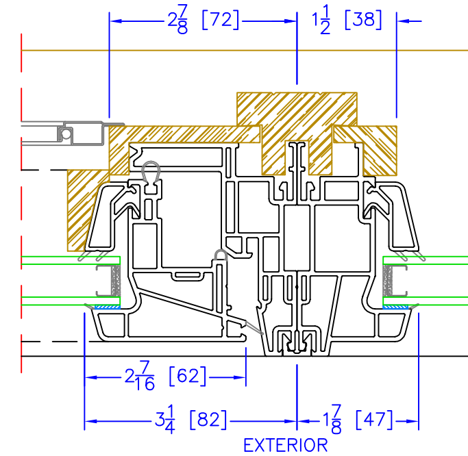
OPERATOR/NARROW PICTURE (PN) VERTICAL/HORIZONTAL MULLION
