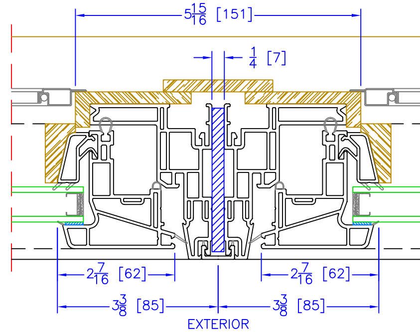
OPERATOR/OPERATOR VERTICAL/HORIZONTAL REINFORCEMENT MULLION
