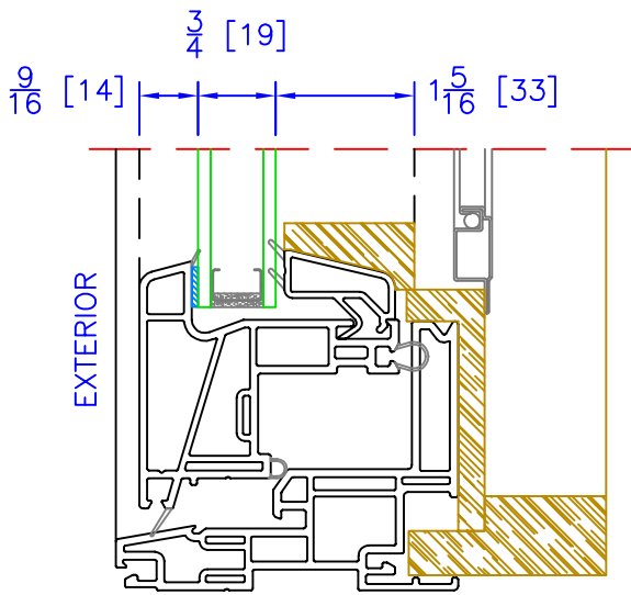
OPERATOR/FIXED DUAL GLAZING OPTION ( \frac{3}{4} " OA)
