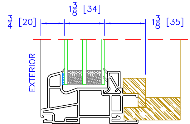
NARROW PICTURE (PN) TRIPLE GLAZING OPTION ( 1\frac{3}{8} " OA)
