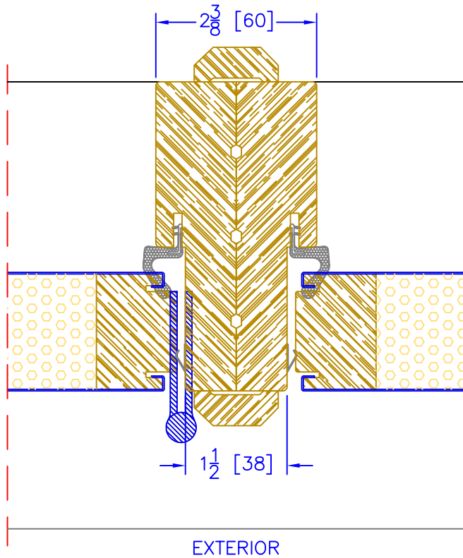
4 5/8" OUTSWING OPERATOR/SIDELITE VERTICAL MULLION
