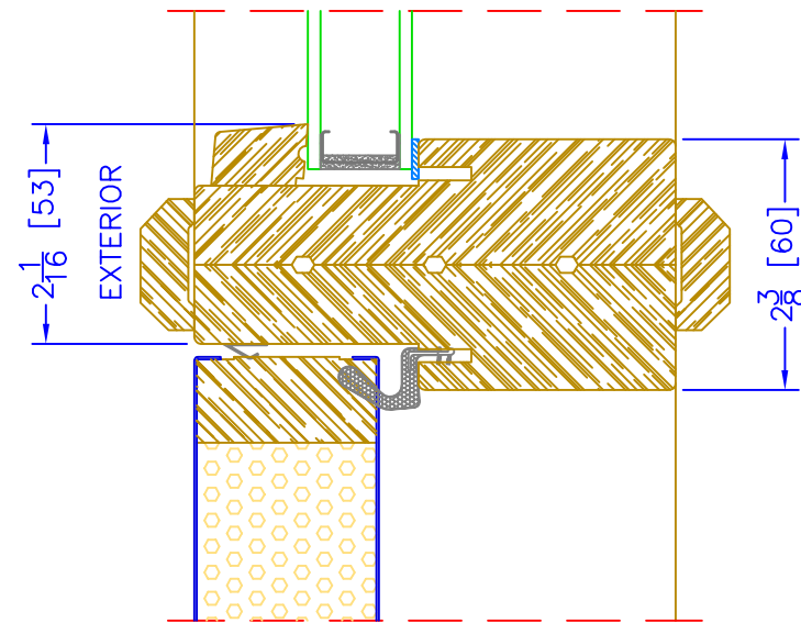
4 5/8" OUTSWING TRANSOM o/ OPERATOR HORIZONTAL MULLION
