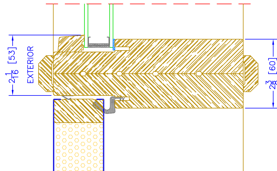
6 5/8" OUTSWING TRANSOM o/ OPERATOR HORIZONTAL MULLION
