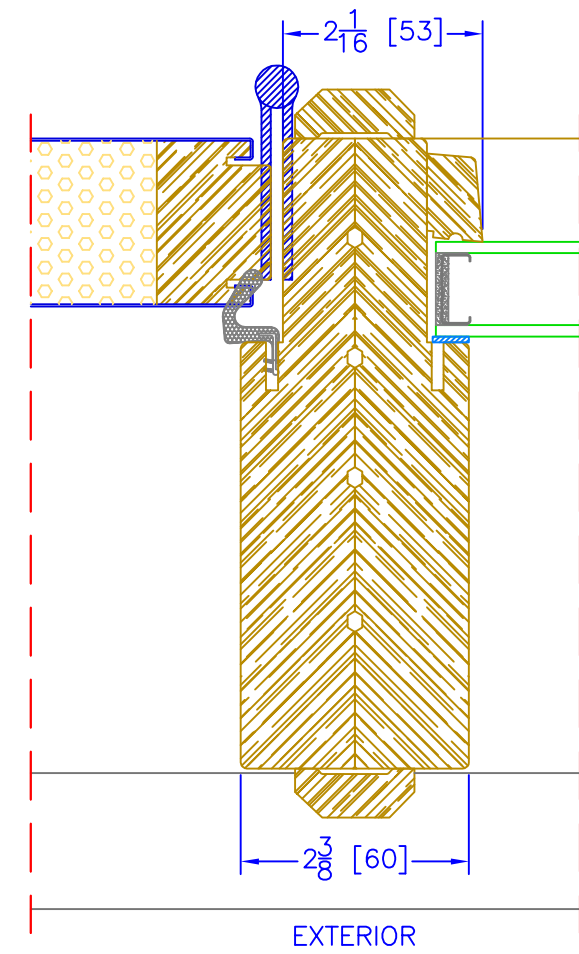
6 5/8" INSWING OPERATOR/S-100 VERTICAL MULLION
