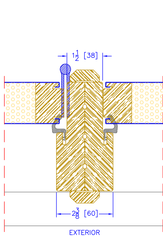
4 5/8" INSWING OPERATOR/SIDELITE VERTICAL MULLION
