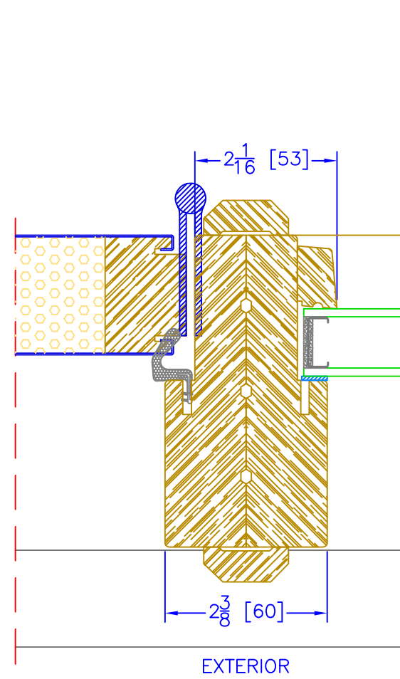
4 5/8" INSWING OPERATOR/S-100 VERTICAL MULLION
