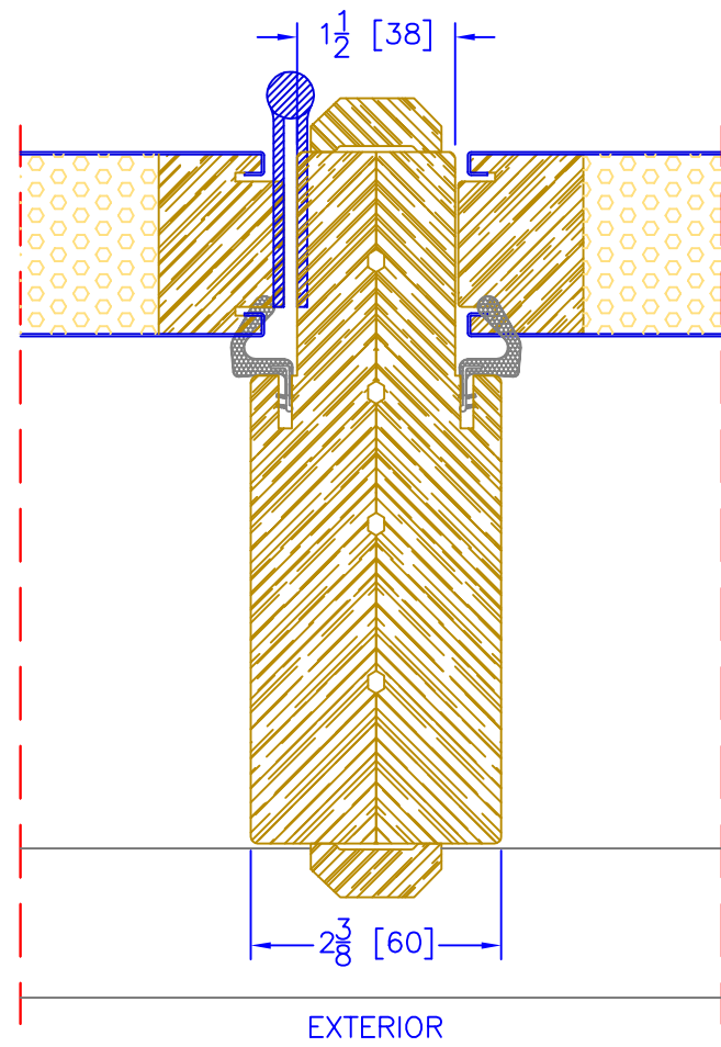
6 5/8" INSWING OPERATOR/SIDELITE VERTICAL MULLION
