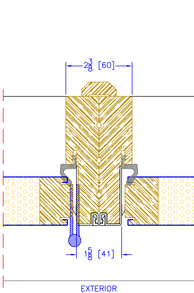
4 5/8" OUTSWING OPERATOR/SIDELITE VERTICAL MULLION
