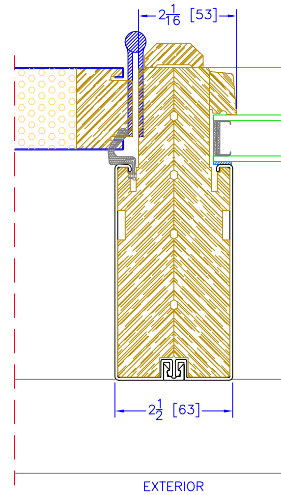
6 5/8" INSWING OPERATOR/S-100 VERTICAL MULLION
