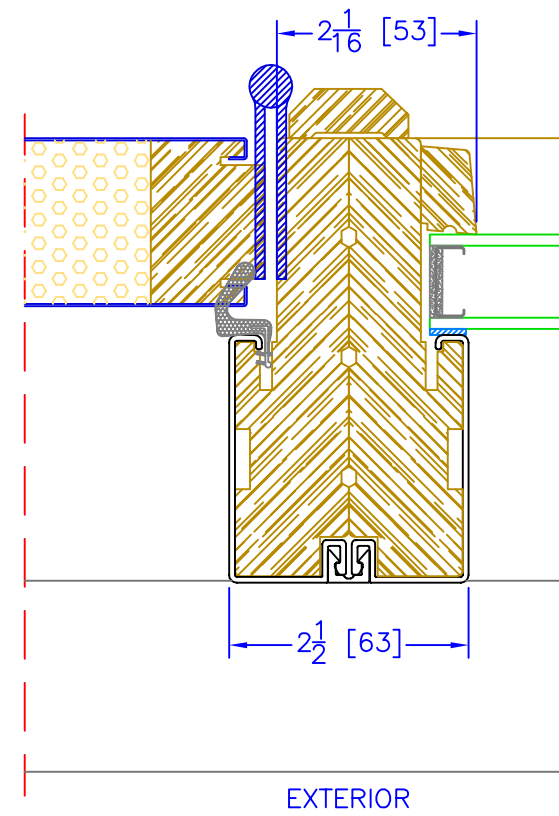
4 5/8" INSWING OPERATOR/S-100 VERTICAL MULLION
