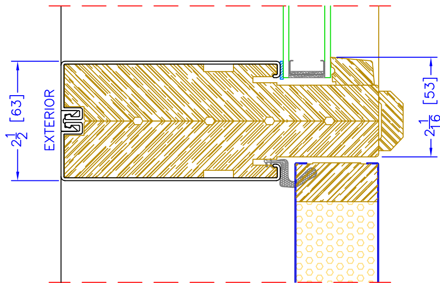
6 5/8" INSWING TRANSM o/ OPERATOR HORIZONTAL MULLION
