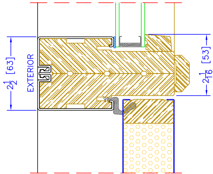
4 5/8" INSWING TRANSM o/ OPERATOR HORIZONTAL MULLION
