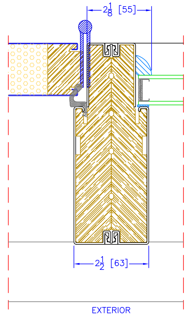
6 5/8" INSWING OPERATOR/S-100 VERTICAL MULLION
