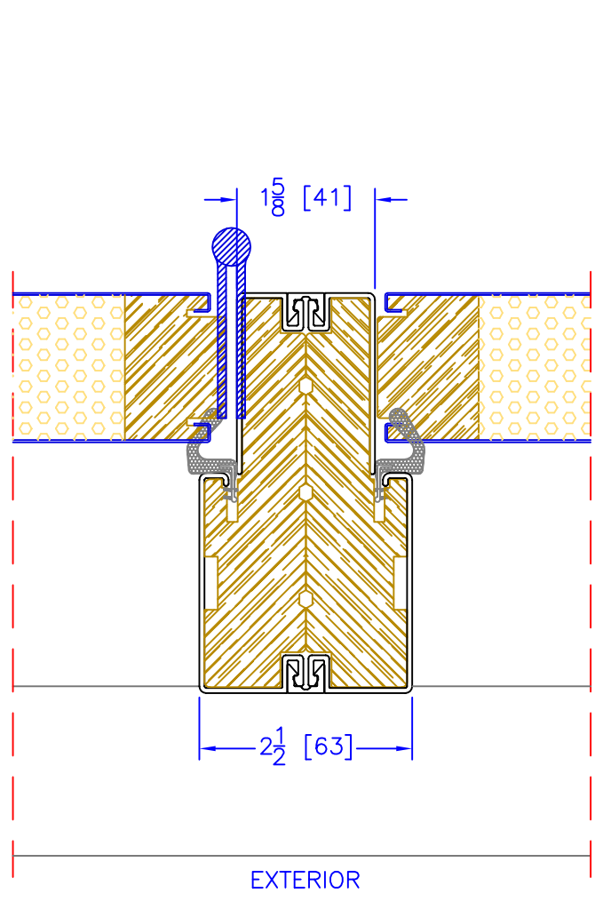
4 5/8" INSWING OPERATOR/SIDELITE VERTICAL MULLION
