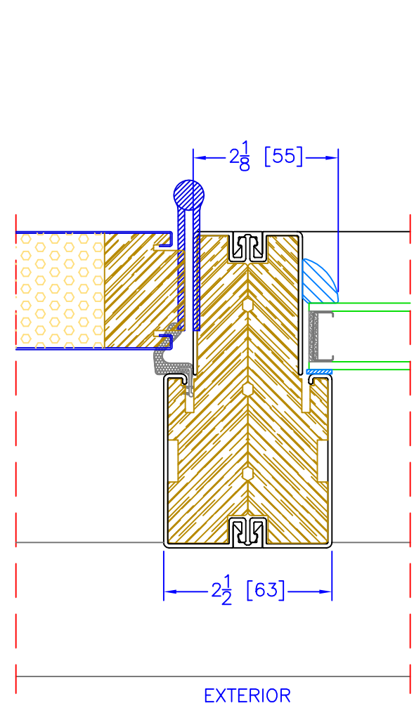
4 5/8" INSWING OPERATOR/S-100 VERTICAL MULLION
