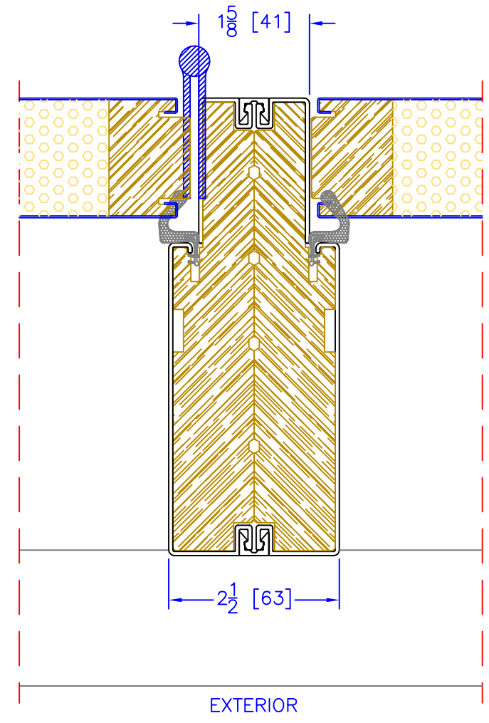
6 5/8" INSWING OPERATOR/SIDELITE VERTICAL MULLION
