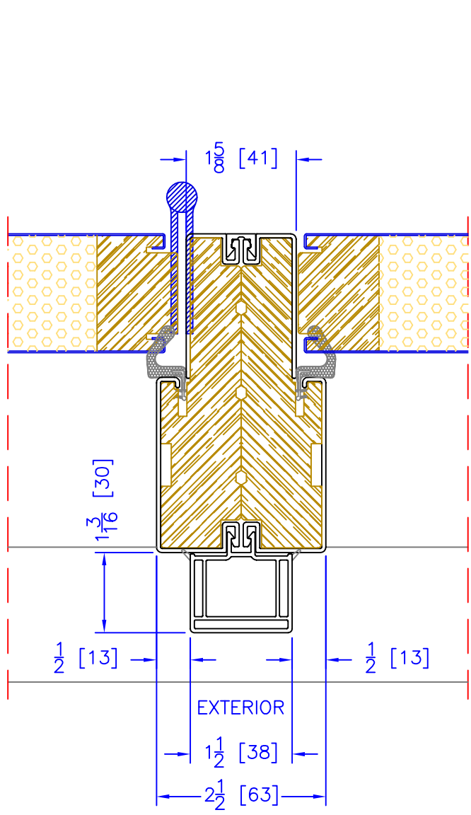
4 5/8" INSWING OPERATOR/SIDELITE VERTICAL MULLION STORM DOOR PREP ON POST ONLY AVAILABLE w/ STORM DOOR PREP BRICKMOULDS
