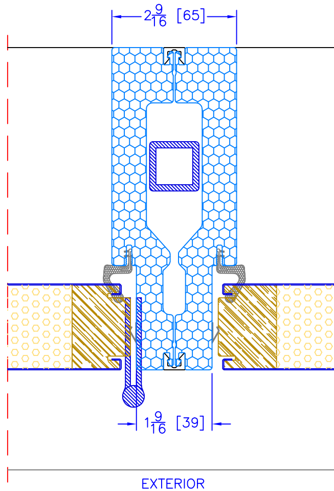
6 5/8" OUTSWING OPERATOR/SIDELITE VERTICAL MULLION
