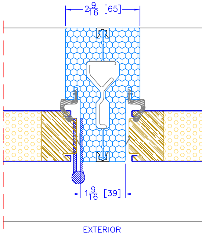
4 5/8" OUTSWING OPERATOR/SIDELITE VERTICAL MULLION
