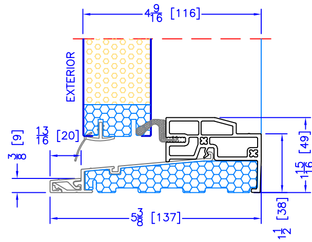
48" OUTSWING HIGH PERFORMANCE SILL CLOSE-OUT EXTENSION (USED WITH PLAIN FRAME)
