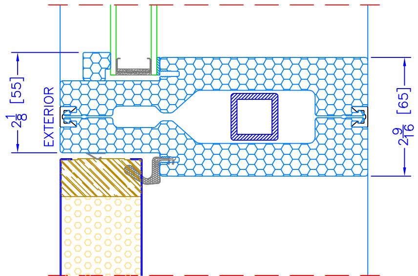
6 5/8" OUTSWING TRANSOM/SHAPE o/ OPERATOR HORIZONTAL MULLION
