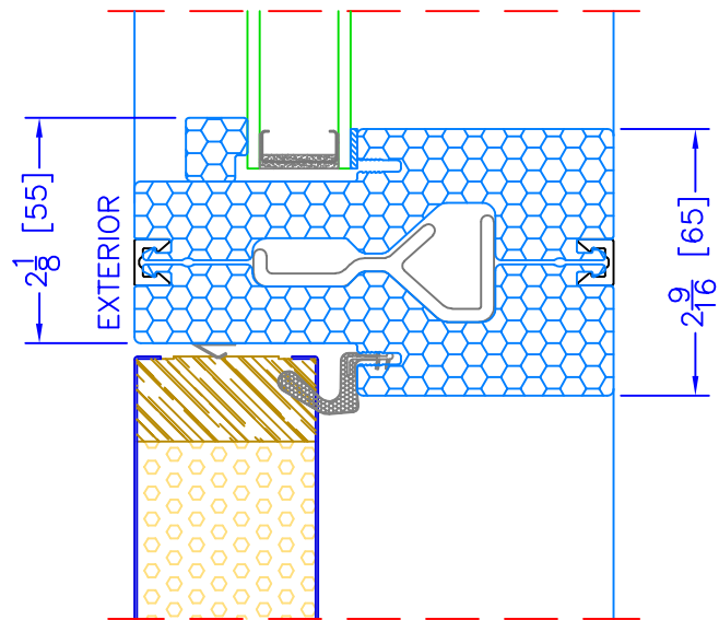
4 5/8" OUTSWING TRANSOM/SHAPE o/ OPERATOR HORIZONTAL MULLION
