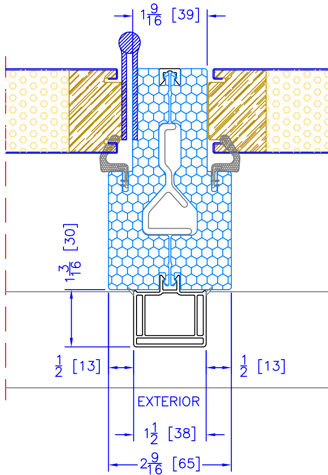
4 5 / 8 " INSWING OPERATOR/SIDELITE VERTICAL MULLION STORM DOOR PREP ON POST ONLY AVAILABLE w/ STORM DOOR PREP BRICKMOULDS
