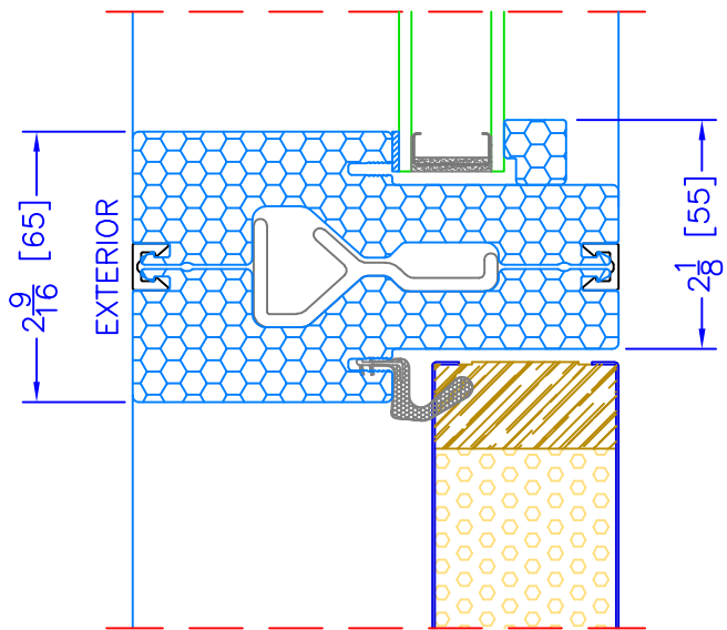
4 5 / 8 " INSWING TRANSOM/SHAPE o/ OPERATOR HORIZONTAL MULLION
