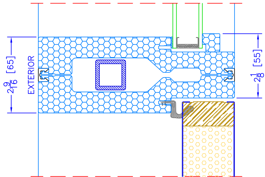
6 5 / 8 " INSWING TRANSOM/SHAPE o/ OPERATOR HORIZONTAL MULLION
