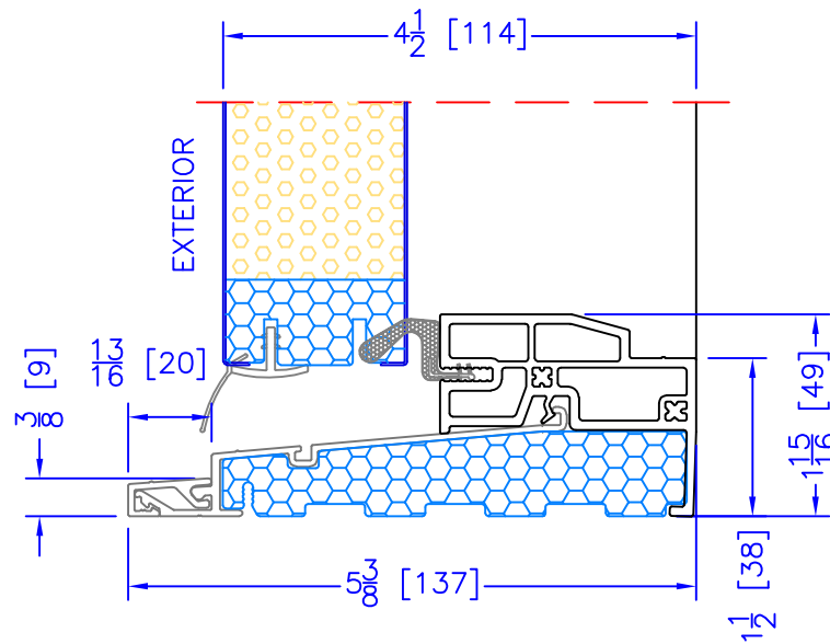
4 1/2" OUTSWING HIGH PERFORMANCE SILL CLOSE-OUT EXTENSION (USED WITH PLAIN FRAME)
