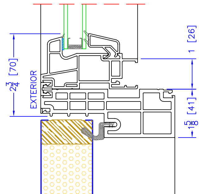
4 1/2" OUTSWING SHAPE o/ OPERATOR HORIZONTAL MULLION
