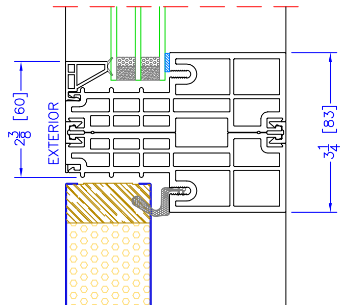
4 1/2" OUTSWING TRANSOM o/ OPERATOR HORIZONTAL MULLION
