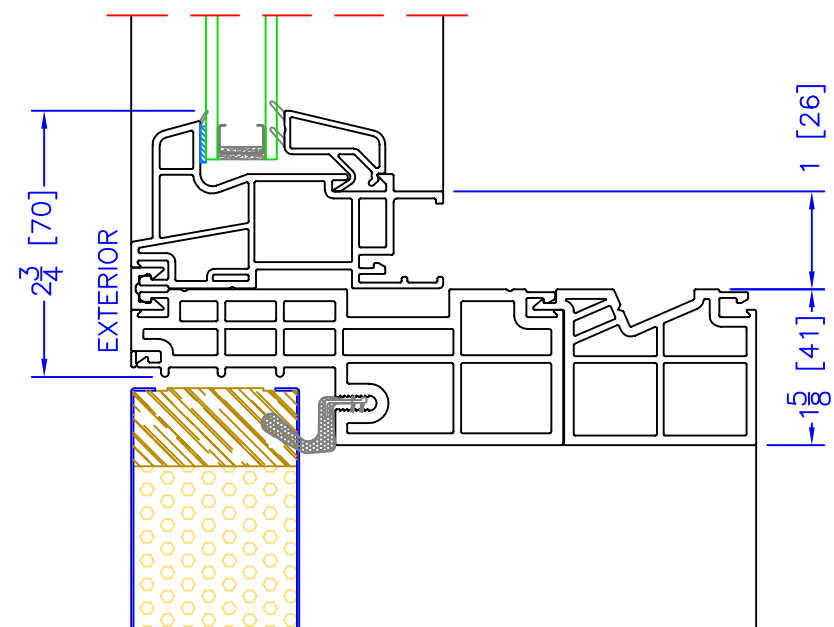
6 1/2" OUTSWING SHAPE o/ OPERATOR HORIZONTAL MULLION
