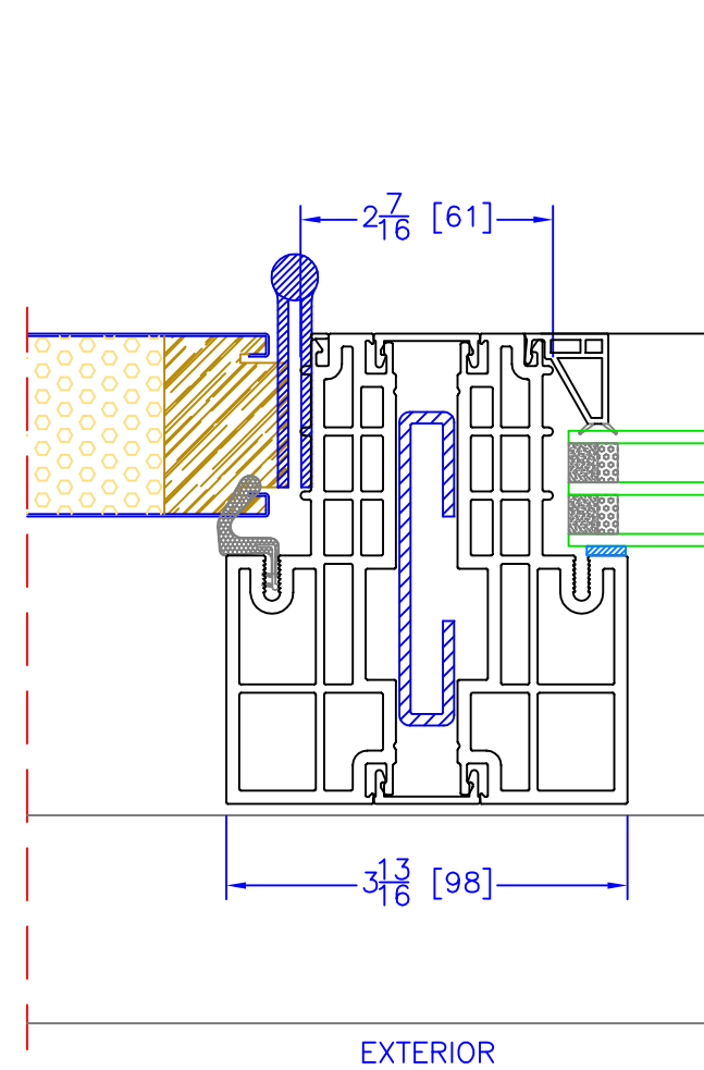
4 1/2" INSWING OPERATOR/S-100 VERTICAL MULLION
