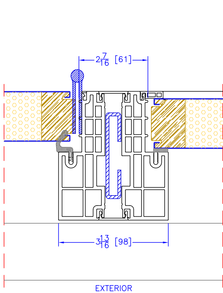
4 1/2" INSWING OPERATOR/SIDELITE VERTICAL MULLION
