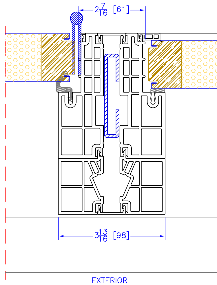
6 1/2" INSWING OPERATOR/SIDELITE VERTICAL MULLION
