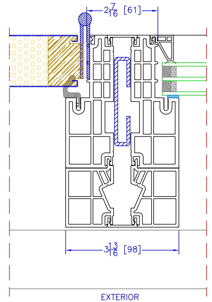
6 1/2" INSWING OPERATOR/S-100 VERTICAL MULLION
