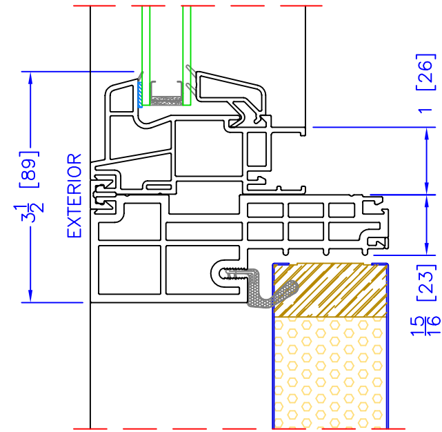
4 1/2" INSWING SHAPE o/ OPERATOR HORIZONTAL MULLION
