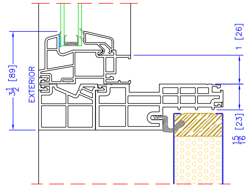
6 1/2" INSWING SHAPE o/ OPERATOR HORIZONTAL MULLION
