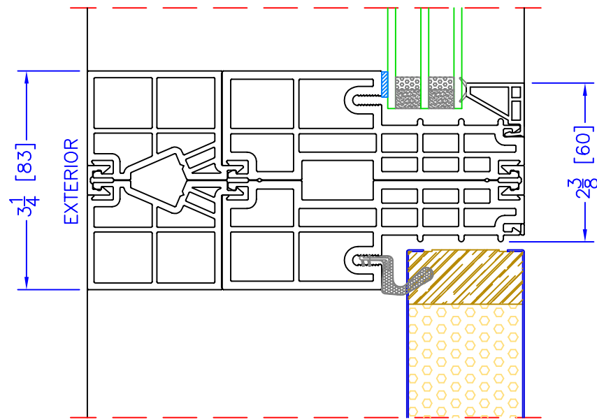
6 1/2" INSWING TRANSOM o/ OPERATOR HORIZONTAL MULLION
