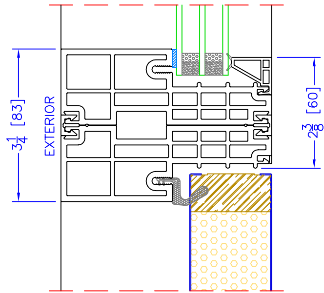
4 1/2" INSWING TRANSOM o/ OPERATOR HORIZONTAL MULLION
