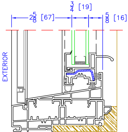
OPERATOR DUAL GLAZING OPTION ( \frac{3}{4} " OA)
