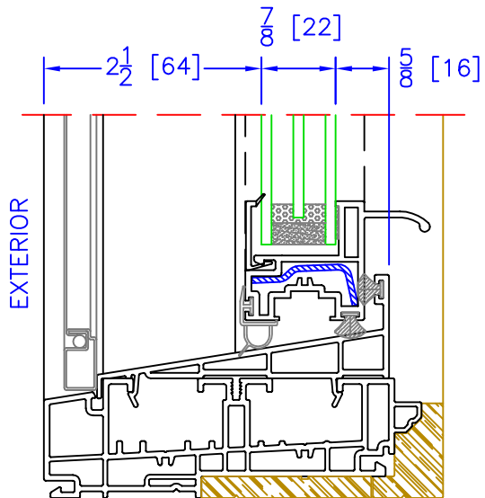
OPERATOR TRIPLE GLAZING OPTION ( \frac{7}{8} " OA)
