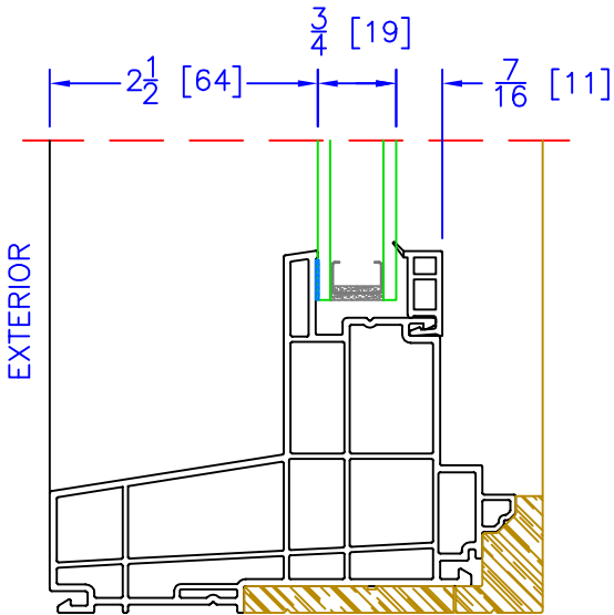
FIXED DUAL GLAZING OPTION ( \frac{3}{4} " OA)
