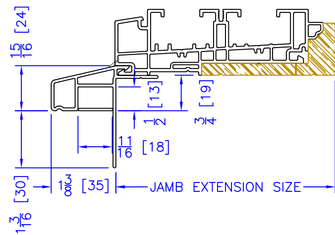
7/8" BM/J-TRIM
