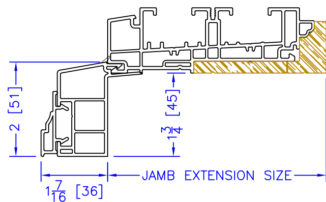
2" 2-PC CONTOUR BM
