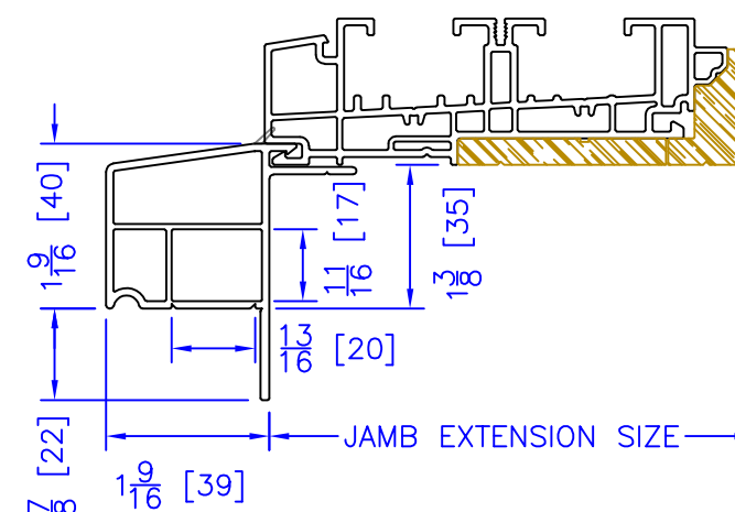
SILL BM
