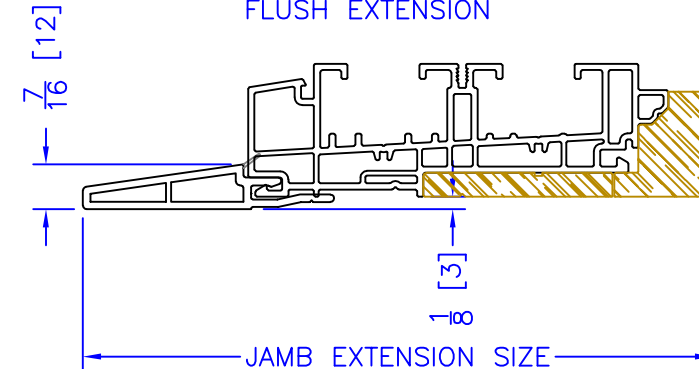
FLUSH EXTENSION
