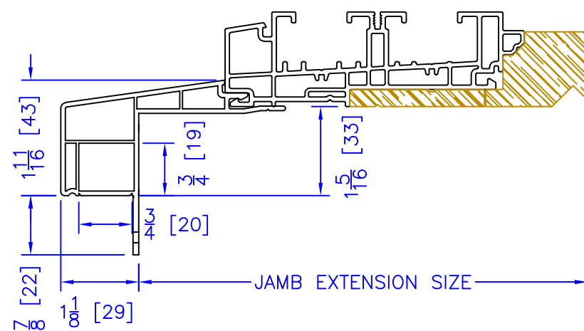
1-1/2" EXTENDED BM/J-TRIM
