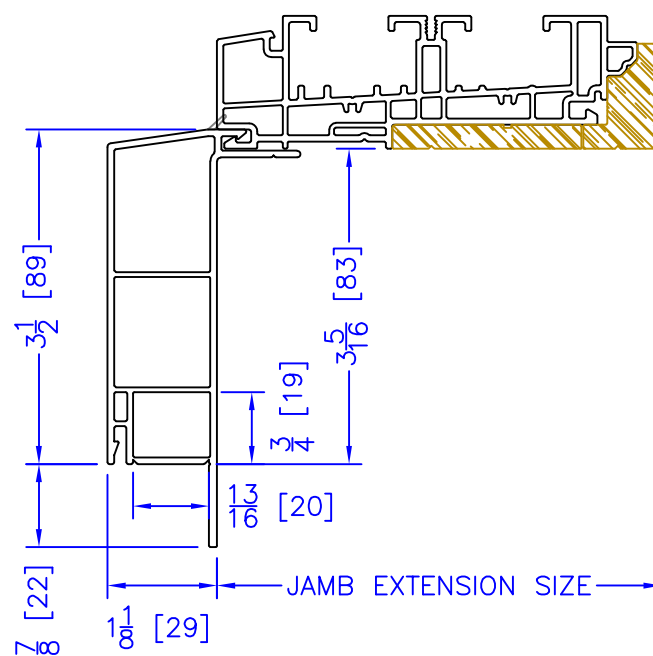
3-1/2" BM/J-TRIM
