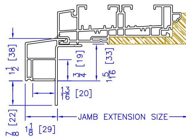
1-1/2" BM/J-TRIM
