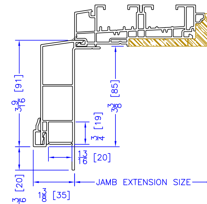
3-1/2" 180 BM/J-TRIM
