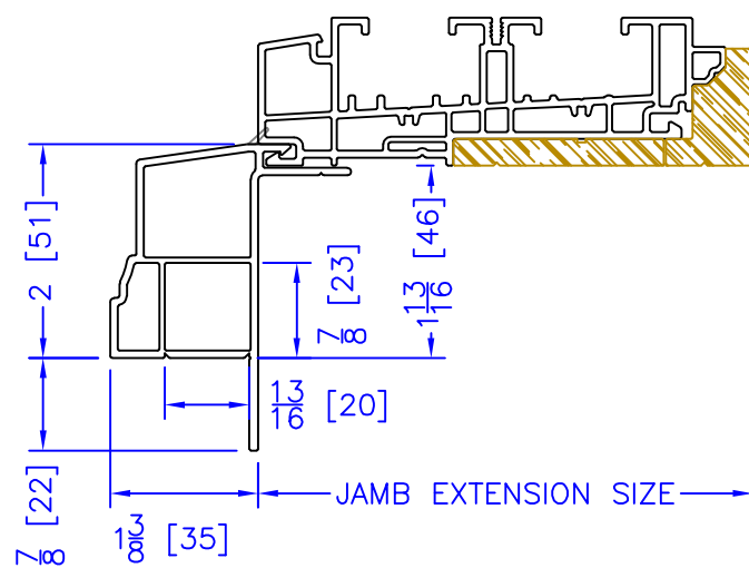
2" 180 BM/J-TRIM
