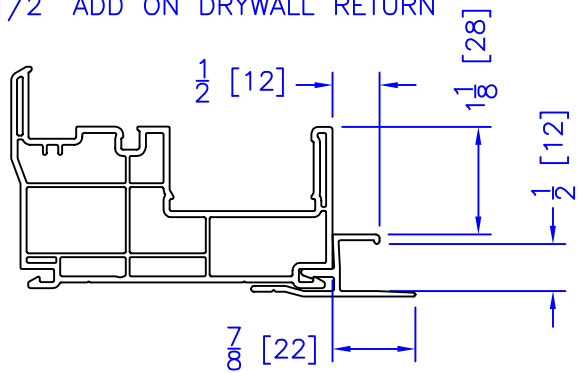
1/2" ADD ON DRYWALL RETURN
