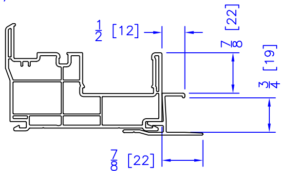
3/4" ADD ON DRYWALL RETURN
