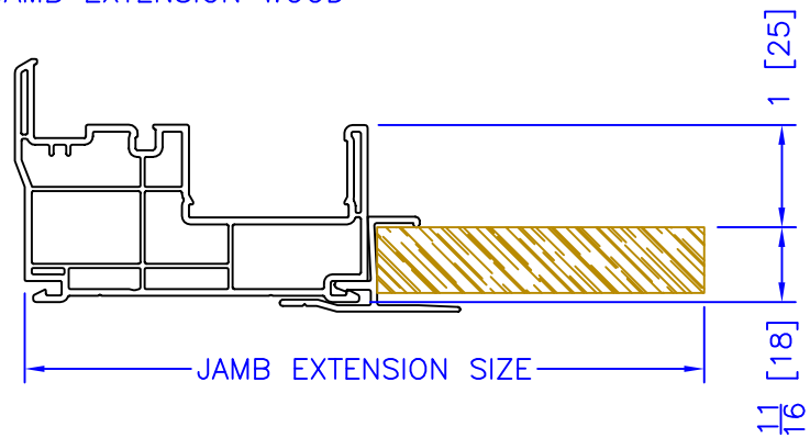
JAMB EXTENSION WOOD
