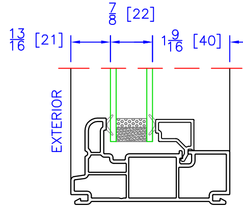
NARROW PICTURE (PN) DUAL GLAZING OPTION ( \frac{7}{8} " OA)
