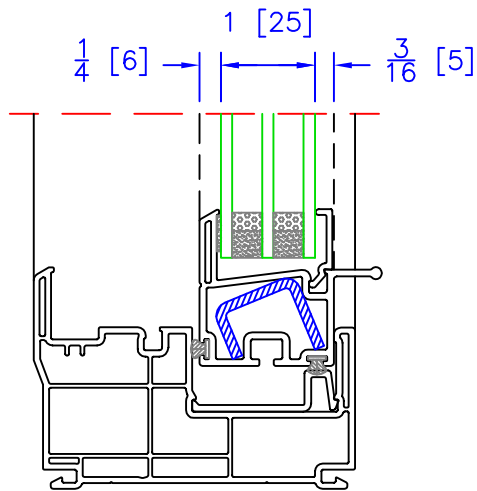
OPERATING SASH TRIPLE GLAZING OPTION (1" OA)
