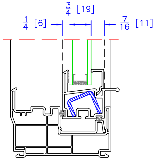
OPERATING SASH DOUBLE GLAZING OPTION ( \frac{3}{4} " OA)
