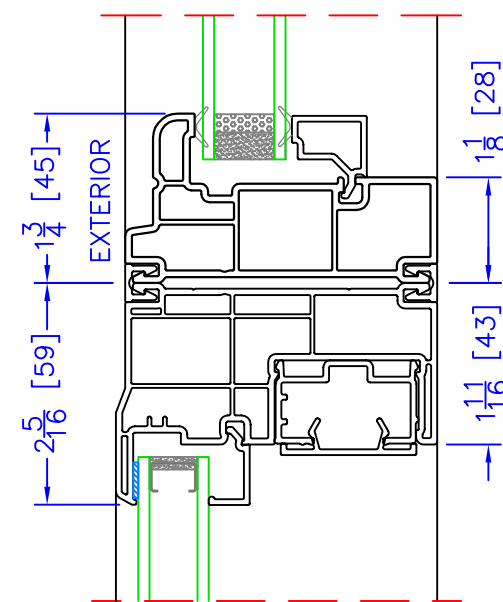
NARROW PICTURE (PN)/OPERATOR HORIZONTAL MULLION
