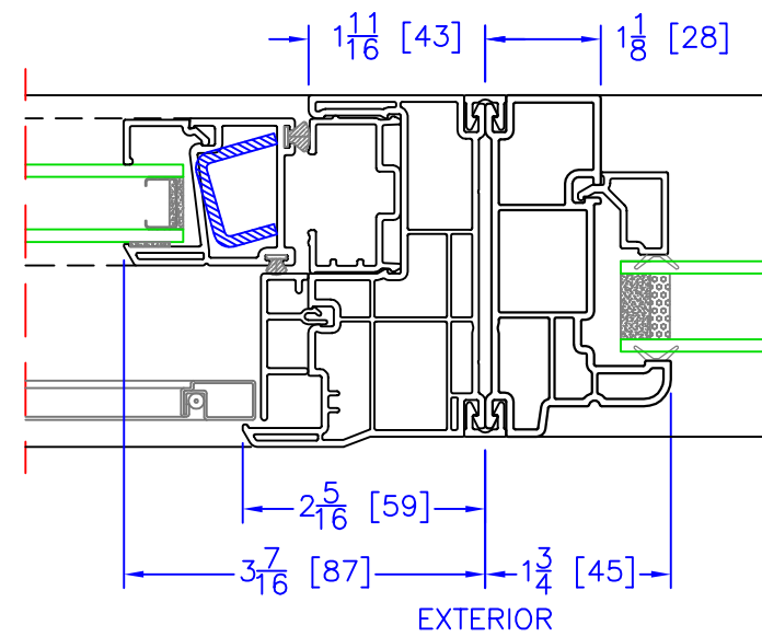
EXTERIOR OPERATOR (BOTTOM SASH)/NARROW PICTURE (PN) VERTICAL MULLION
