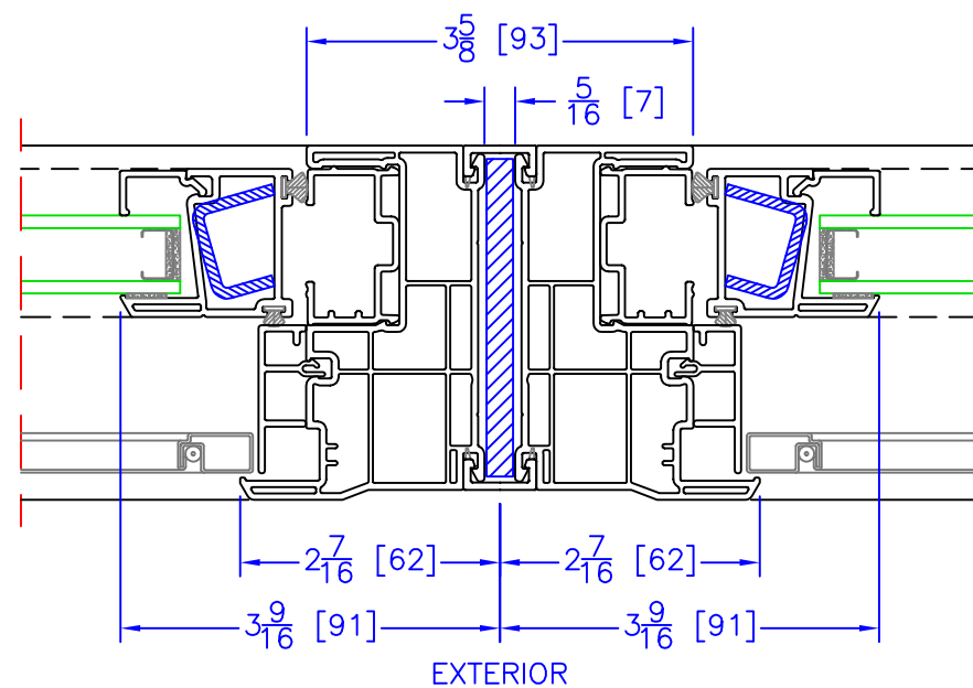
EXTERIOR OPERATOR (BOTTOM SASH)/OPERATOR (BOTTOM SASH) VERTICAL REINFORCEMENT MULLION
