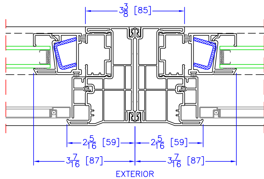
EXTERIOR OPERATOR (BOTTOM SASH)/OPERATOR (BOTTOM SASH) VERTICAL MULLION
