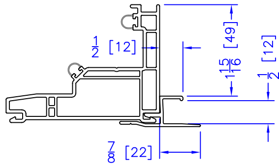
1/2" ADD ON DRYWALL RETURN
