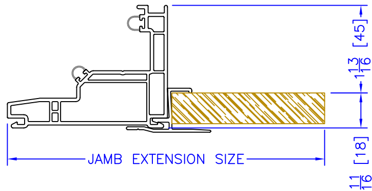
JAMB EXTENSION WOOD
