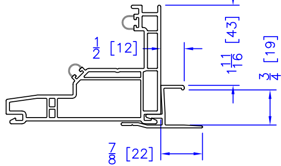
3/4" ADD ON DRYWALL RETURN
